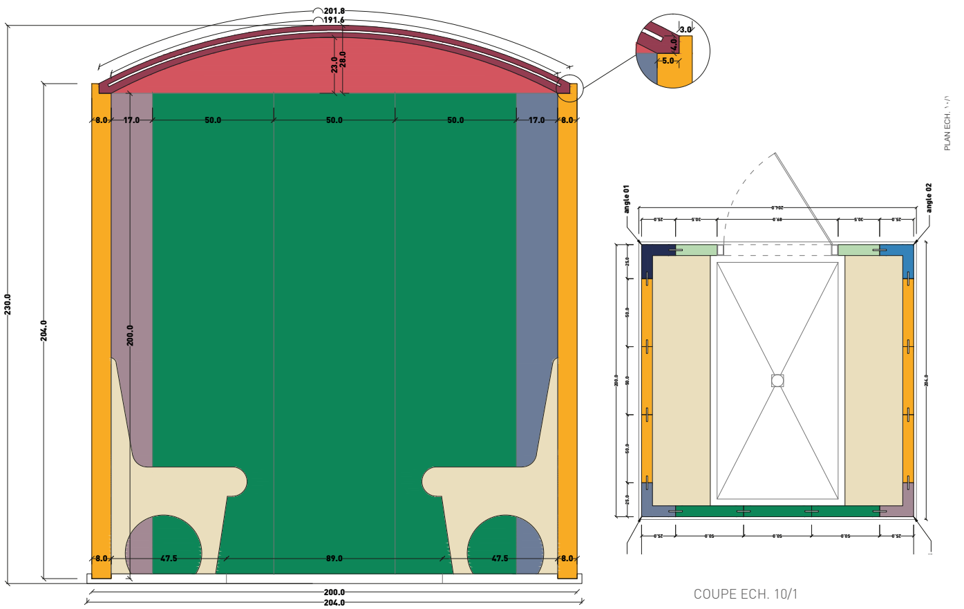
EXAMPLE OF PLAN Custom-made plans by an architect
